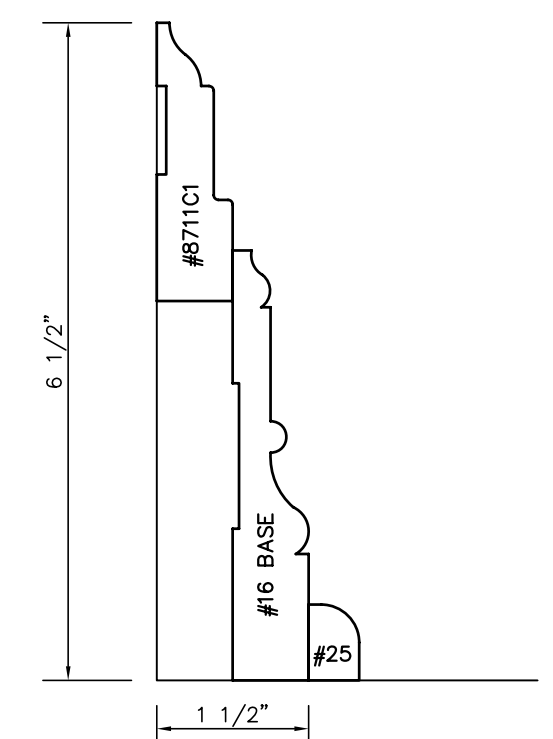
6 1/2" BASE FOR 9' CEILING
