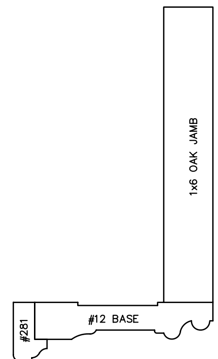
TYPICAL DOOR & WINDOW TRIM EXCEPT DOOR & WINDOWS WITH ELLIPTICAL TRANSOM
