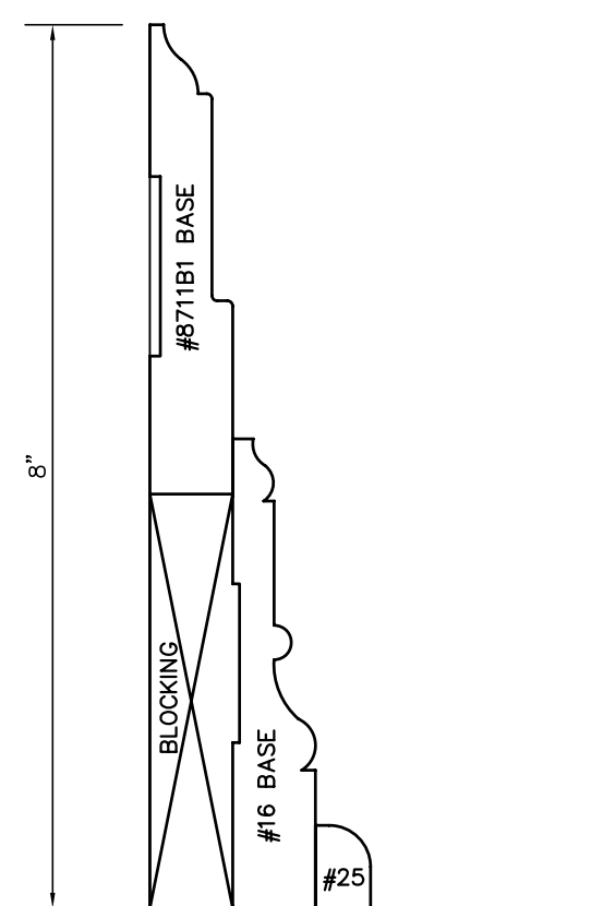
8" BASE FOR 10' CEILING AREAS
