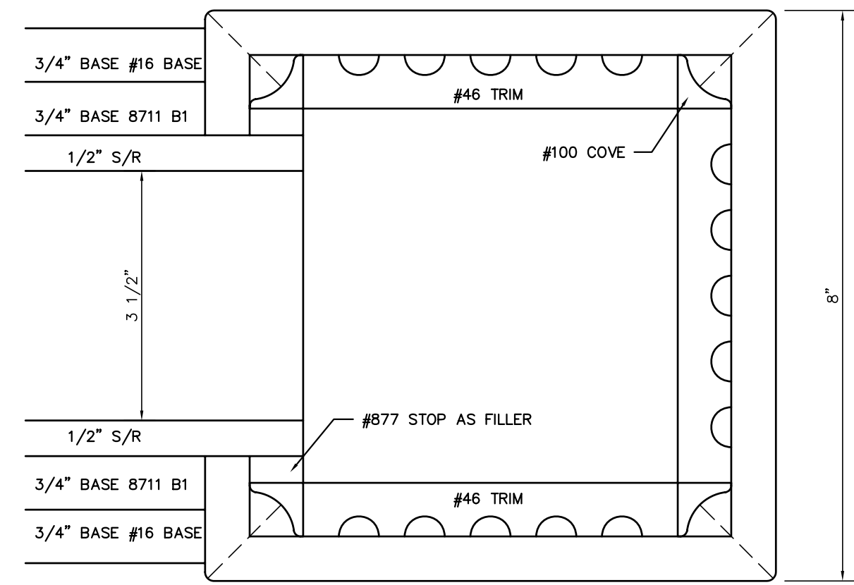
DETAIL FOR 8' CASSED OPENINGS
